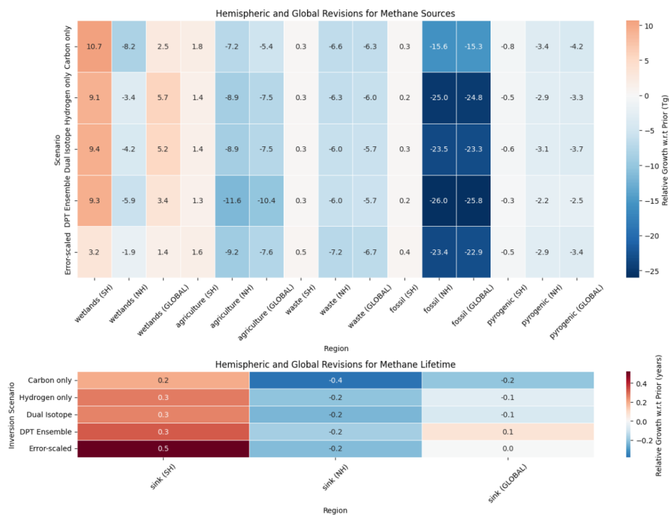
645 Fig. 5: Top panel: Hemispheric and global revisions w.r.t the priors ( Growth_{posterior} - Growth_{prior} ) of the growth in emissions by sector (wetlands, agriculture, waste, fossil, pyrogenic) in teragrams (Tg) per year. Growth is defined as the difference between the 1993-95 and 2021-23 averages. Bottom panel: hemispheric and global revisions for CH_4 lifetime (in years). The \chi(CH_4) -only inversion (using mole fraction data without isotopic constraints) is shown in SI section 12. This inversion yields unrealistic source partitioning due to a lack of isotopic information to distinguish between biogenic and thermogenic sources, 650 underscoring the need for isotopic constraints to achieve robust source attribution.
